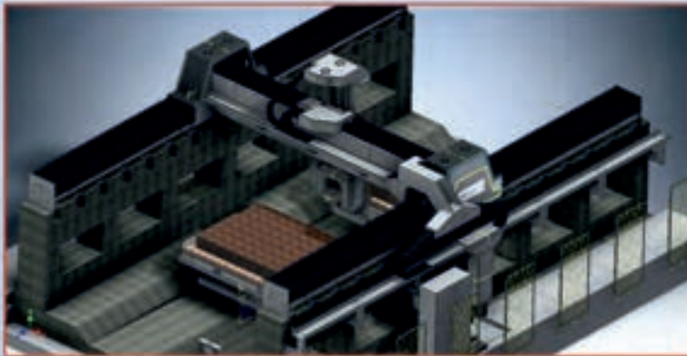
CNC/NC/PLC 3-4-5 EKSEN 12 M. GANTRY TİP 3 TABLALI KÖPRÜ KESİM MAKİNASI - POWER BRIDGE M1200 CNC/NC/PLC 3-4-5 AXES 12 Meter ( GANTRY ) TYPE BRIDGE CUTTING MACHINE
